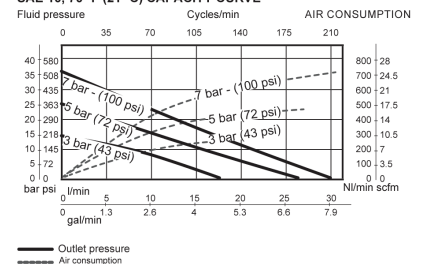
SAE 10, 70 °F (21 °C) CAPACITY CURVE
